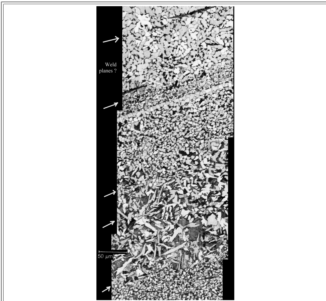
Upper part of the scan through the animal part of the left head. Possible welding planes (more or less perpendicular to the screen) are indicated. Note the sharp but featureless transitions between regions of different grain size and structure, and the presence of elongated slag inclusions nearby in some cases.
