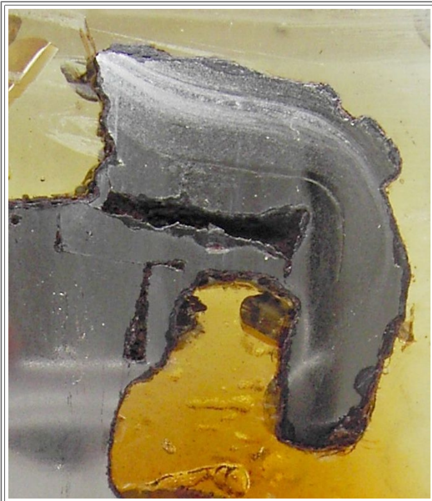
Part of Kiel half; polished and Nital etched. Strongly contrast enhanced.
